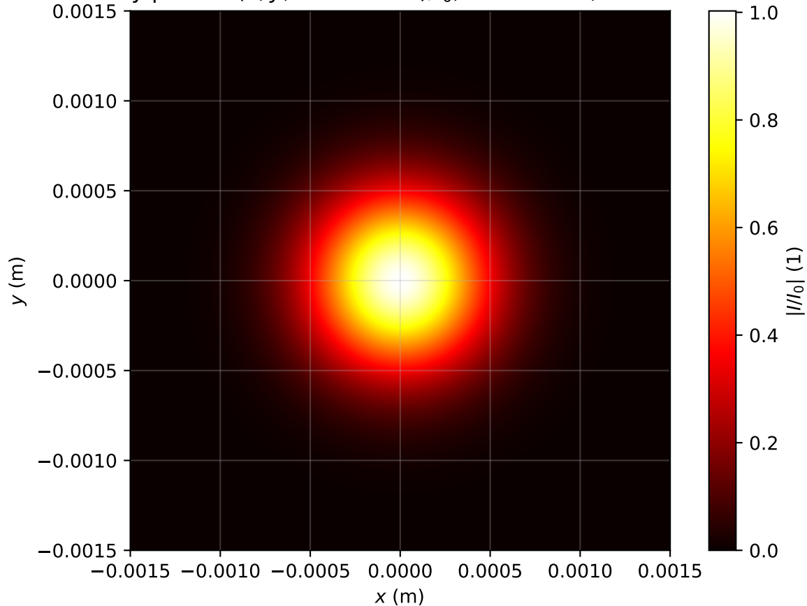
Intensity profile I(x, y, z = 0.318m)/I_0 , Pin=0.3Pcr, artificial time
